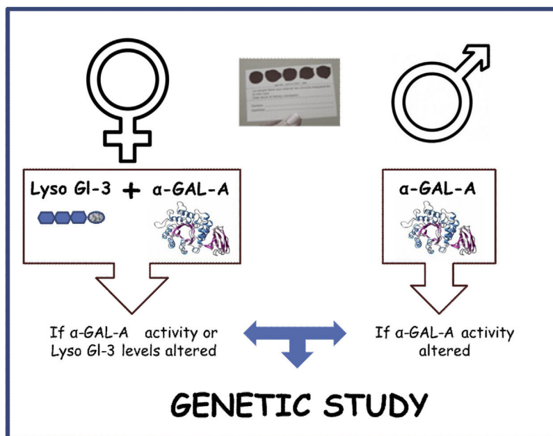
Fig. 1 – Diagnostic algorithm.
