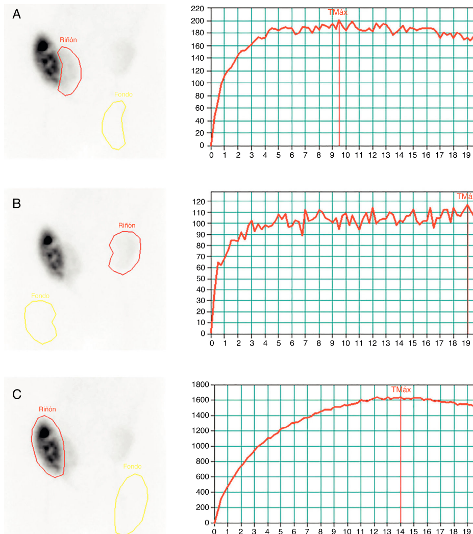
Fig. 2 – ^{99m}\text{Tc} -MAG 3 renogram curves were generated after drawing whole-kidney and background regions of interest for each renal transplant. The results obtained were expressed as the maximum count ratios: 200 cps (A), 117 cps (B) and 1640 cps (C), respectively. The relative differential function showed the following distribution of 16% for the right medial graft (A), 9% for the left graft (B) and 75% for the right lateral graft (C).
