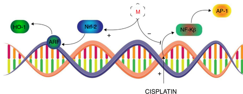
Fig. 2 – Transcriptional control of Melatonin (M) to alleviate cisplatin-induced nephrotoxicity. Melatonin inhibits the cisplatin-induced production of NF- \kappa B and AP-1 while induces the expression of Nrf-2 to mediate the ARF derived activation of HO-1 in alleviation of cisplatin-induced nephrotoxicity.
