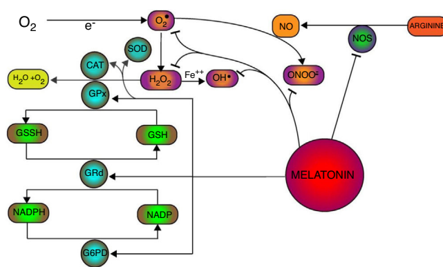
Fig. 1 – Antioxidant mechanism of Melatonin in nephrotoxicity; Melatonin attenuate the oxidative stress by direct neutralization of the reactive species (central), induction of endogenous antioxidant enzymes (left) and inhibits the pro-oxidant pathway of nitric oxide synthase (NOS).
