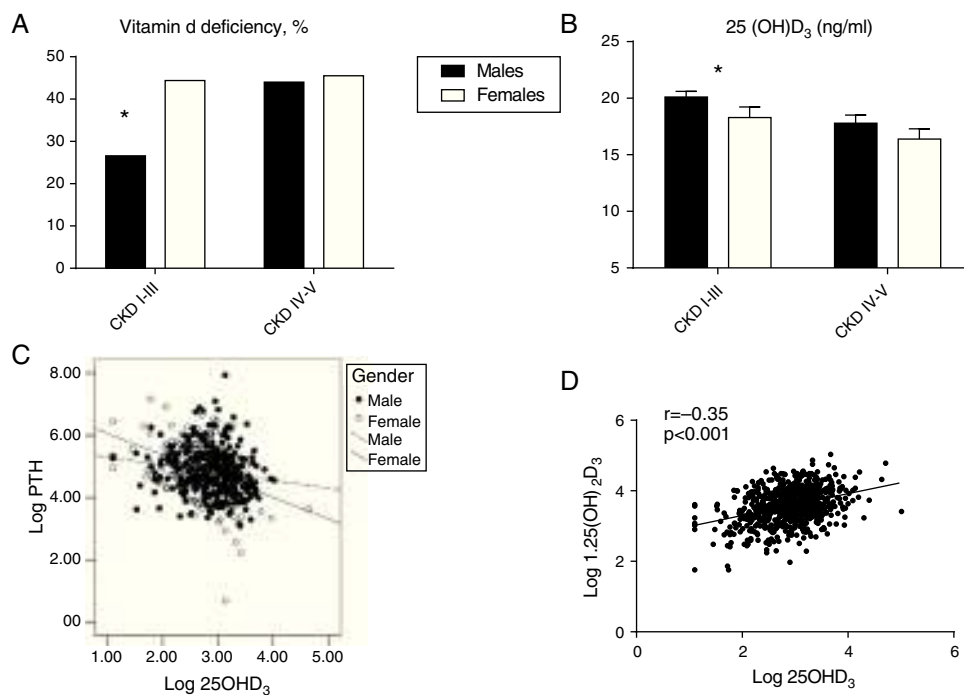
Fig. 3 – Prevalence of Vitamin D deficiency ( 25\text{OHD}_3 < 15 \text{ ng/ml} ) by the CKT-T stage as a function of gender (a). For those recipients who were not treated with vitamin D, 25\text{OHD}_3 by CKD-T stage serum levels (b) and correlation of log transformed 25\text{OHD}_3 with log transformed PTH levels are shown as a function of gender (slope was steeper in women; p = 0.01 ). For all recipients, the correlation between the log transformed 25\text{OHD}_3 and log transformed 1,25(\text{OH})_2\text{D}_3 is shown ( r = -0.35 ; p < 0.001 ) (d). (*) p = 0.003 for the comparison of males vs females in CKD-T Stages I through III; for CKD-T stages IV–V no significant differences between males vs. females.
