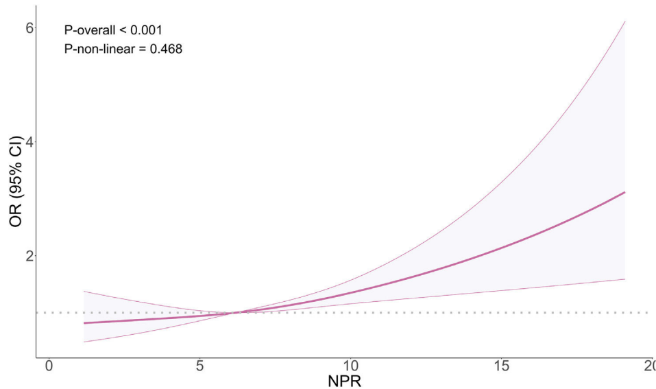
Fig. 2. RCS curve.
