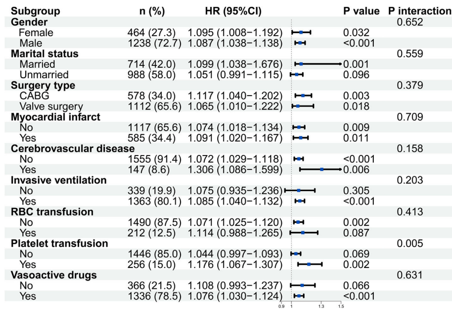
Fig. 3. Subgroup analysis.
